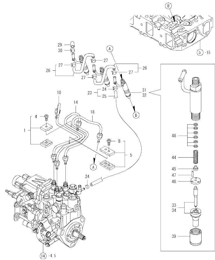
Fig.15. FUEL INJECTION VALVE
