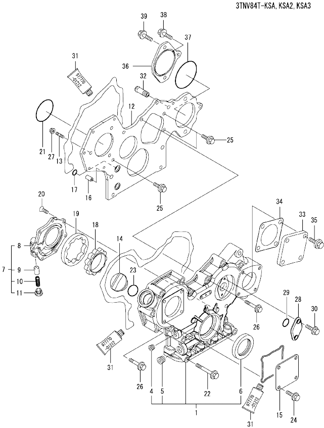
Fig.2. GEAR HOUSING
