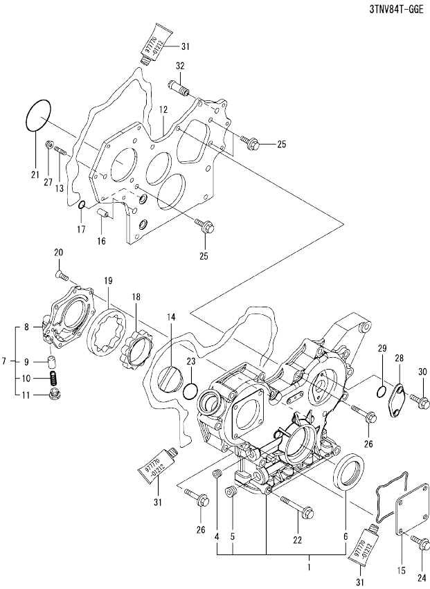
Fig.3. GEAR HOUSING
