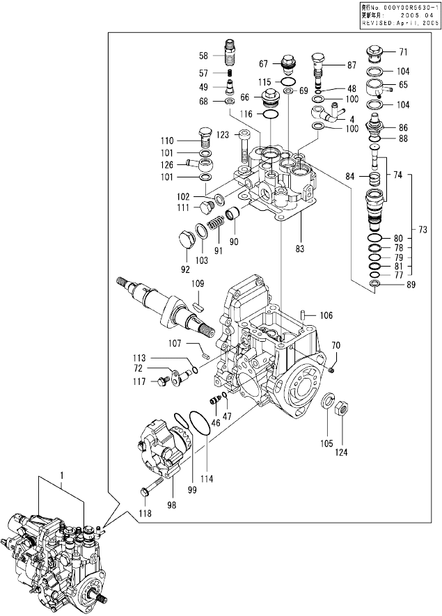
Fig.21. FUEL INJECTION PUMP(INNER PARTS)
