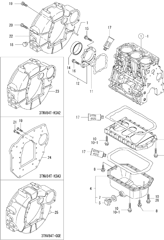
Fig.4. FLYWHEEL HOUSING & OIL SUMP
