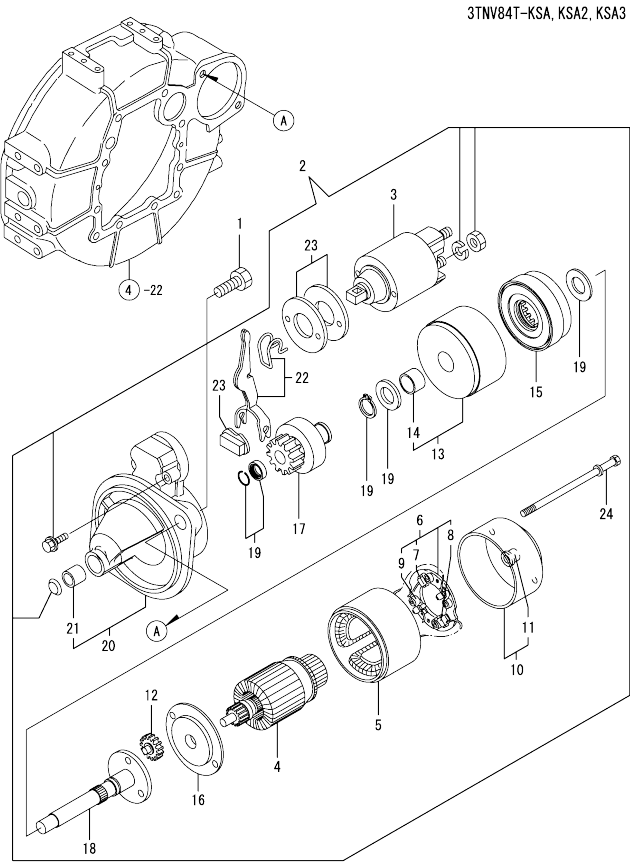
OCR10-M56300 ENGINE Fig.17. STARTING MOTOR
