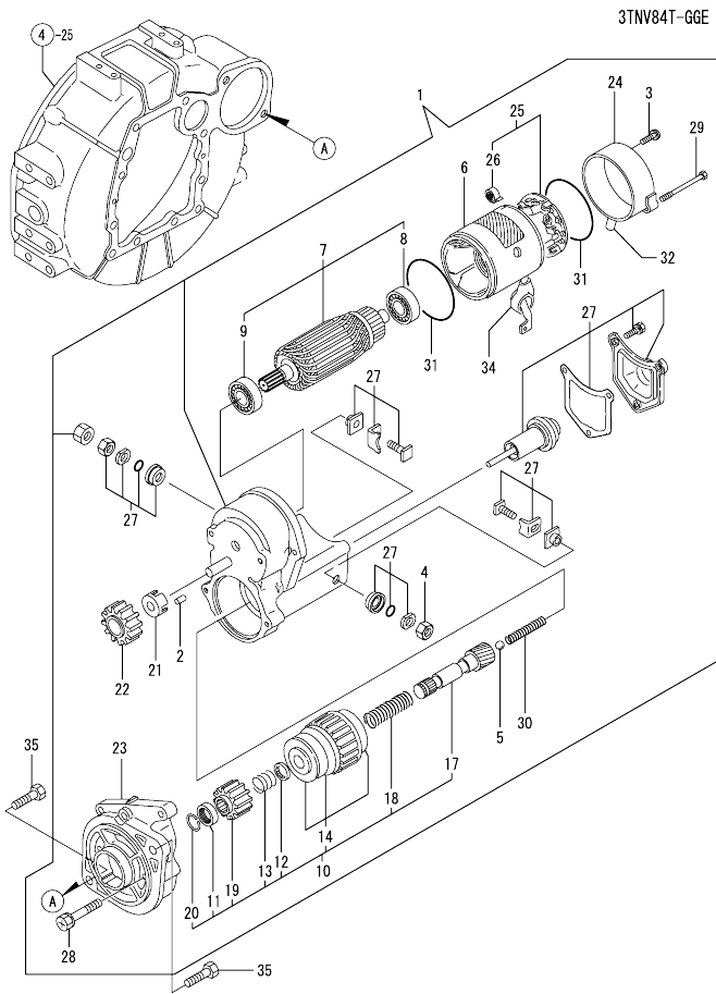
OCR10-M56300 ENGINE Fig.18. STARTING MOTOR
